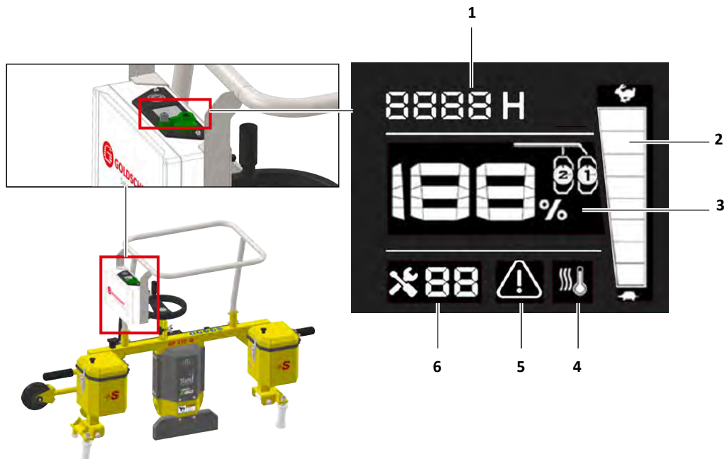
Abb. 2-3 LED-Display
