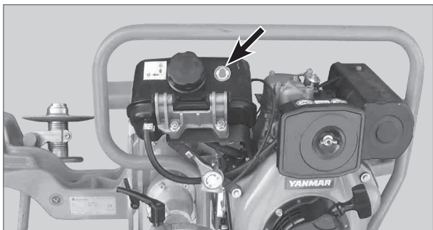
Figure 5: Installation positions for safety signs 2 GP 4000 D
