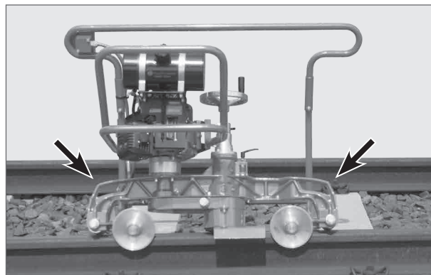
Figure 11: Carrying fixtures
