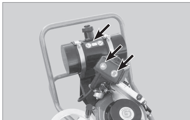
Figure 7: Installation positions for safety signs 2 GP 4000 P
