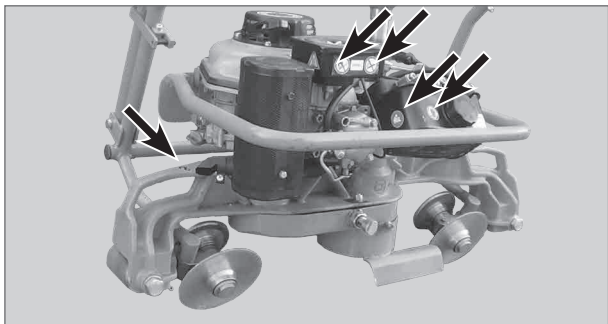
Figure 4: Installation positions for safety signs 1 GP 4000 D
