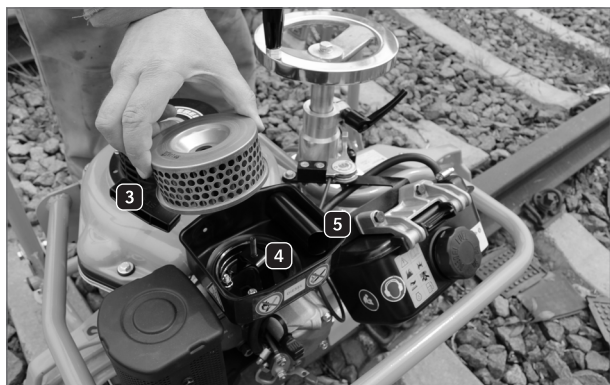
Figure 32: GP 4000 D – Check the air filter 2
