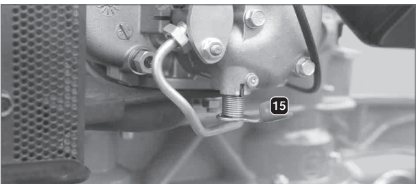
Figure 19: Operating and adjustment controls for diesel engine 2
